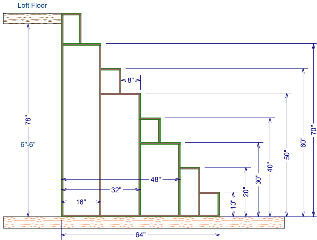
10" Riser with an 8" Tread 3/4" Plywood
