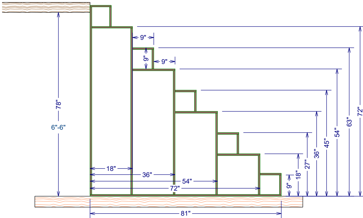
9" Riser with a 9" Tread 3/4" Plywood
